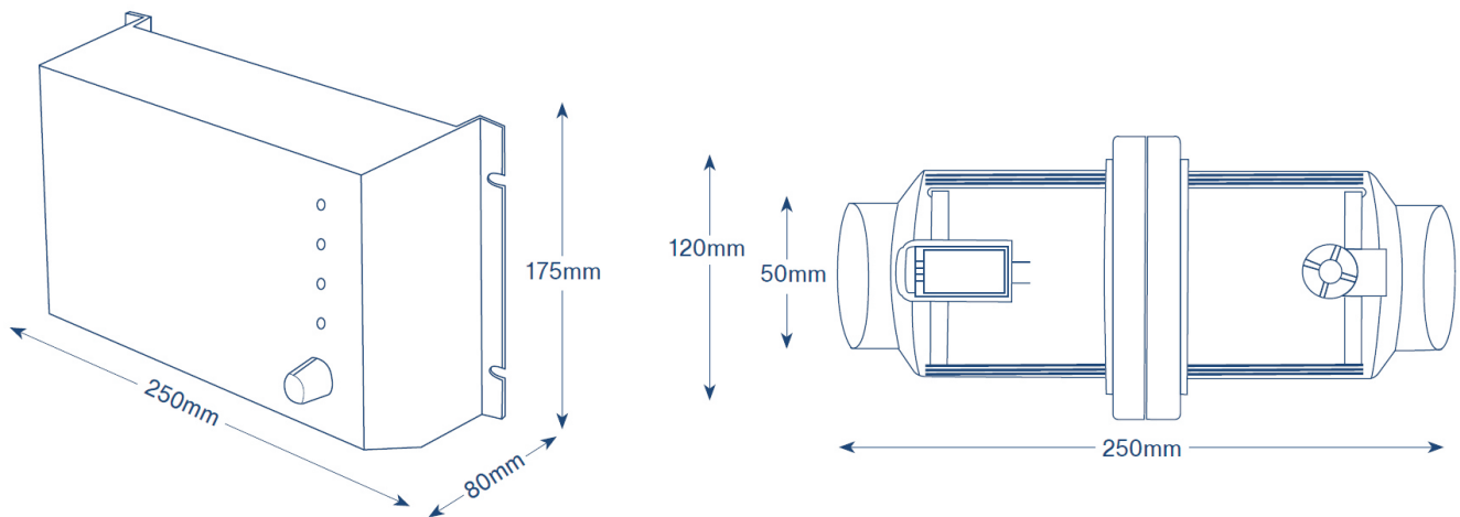
BADU®Logic range power pack dimension table (cm) / BADU®Logic-afmetingstabel (cm)
